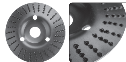
Fig. 15, Rasping discs
