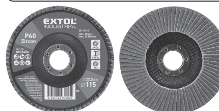
Fig. 14, Flap disc
